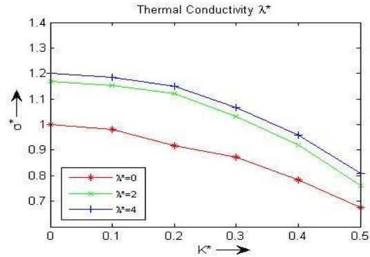
Fig. 1. The growth rate of instability is plotted against the dimensionless wave number k^* with variation in the thermal conductivity \lambda^* = 0, 2, 4 , with taking the values k_s^*, v^*, k_1^* and \tau^* as unity
