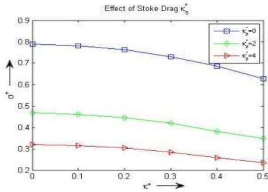
Fig. 6. The growth rate of instability is plotted against the dimensionless wave number k^* with variation in the Stokes' drag constant k_s^* = 0, 2, 4 , with taking the values of \lambda^*, V^*, \nu_0^*, f^*, \nu^* and \tau^* as unity
