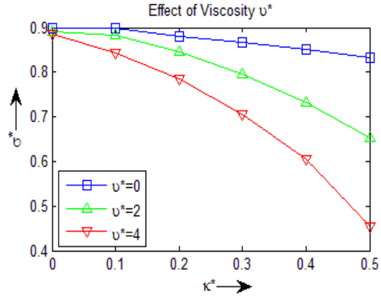
Fig. 4. The growth rate of instability is plotted against the dimensionless wave number k^* with variation in the viscosity \nu^* = 0, 2, 4 , with taking the values of \lambda^*, k_1^*, k_s^* and \tau^* as unity
