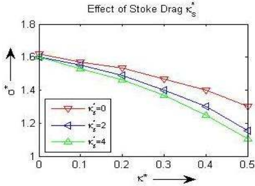
Fig. 3. The growth rate of instability is plotted against the dimensionless wave number k^* with variation in the Stokes' drag constant k_s^* = 0, 2, 4 , with taking the values of \lambda^*, \nu^*, k_1^* and \tau^* as unity
