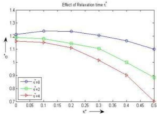
Fig. 5. The growth rate of instability is plotted against the dimensionless wave number k^* with variation in the relaxation time \tau^* = 0, 2, 4 , with taking the values of k_s^*, V^*, \nu_0^*, \vartheta^*, f^* and \lambda^* as unity
