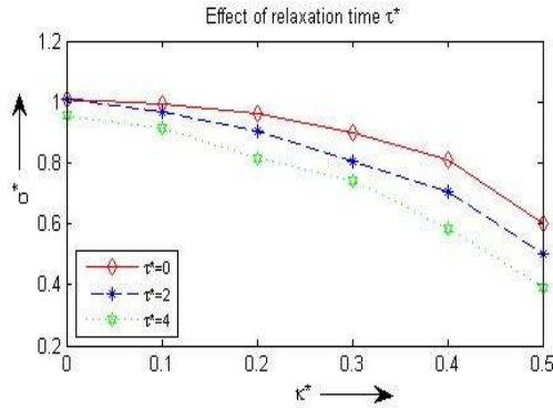
Fig. 2. The growth rate of instability is plotted against the dimensionless wave number k^* with variation in the relaxation time \tau^* = 0, 2, 4 , with taking the values of k_s^*, \nu^*, k_1^* and \lambda^* as unity
