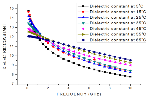
Fig. 1. The graph of dielectric constant against the frequency. The dielectric constant of EMIM-BF 4 decrease when the temperature increased beyond 0.1GHz (i.e. 14.733 to 12.090 for 5°C and 65°C respectively). However, as the frequency increase beyond 0.1GHz the dielectric constant increases when the temperature increases (see Fig.1 above)
