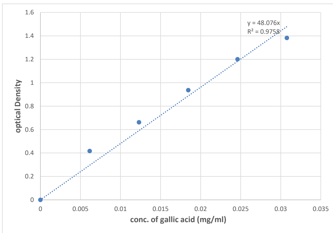
Fig. 2. Calibration curve for determination of total phenolic content
