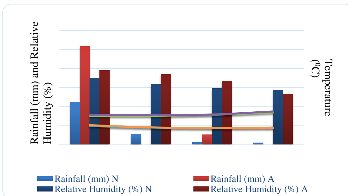
Fig. 1. Meteorological data indicating monthly normal and actual rainfall, relative humidity, maximum and minimum temperature during the cropping period at ZAHRS, Shivamogga
