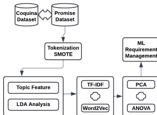
Fig. 3. Flow Diagram for Semantic Analysis Strategies for Agile Requirement Management
