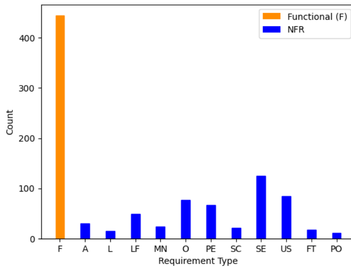
Fig. 1. Promise expanded dataset class distribution
