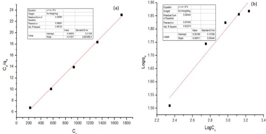
Figure 9; Isotherms graphs: (a) Langmuir isotherm (b) Freundlich isotherm
