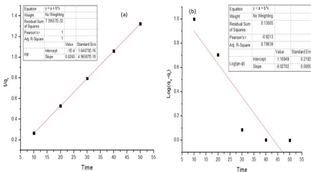
Fig. 8. Kinetics; (a) Pseudo second order (b) Pseudo first order
