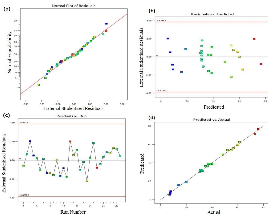
Fig. 4. Diagnostic statistics, (a); Normal plot residuals, (b); Residuals vs predicted, (c); Residuals vs run and (d); Predicted vs actual
