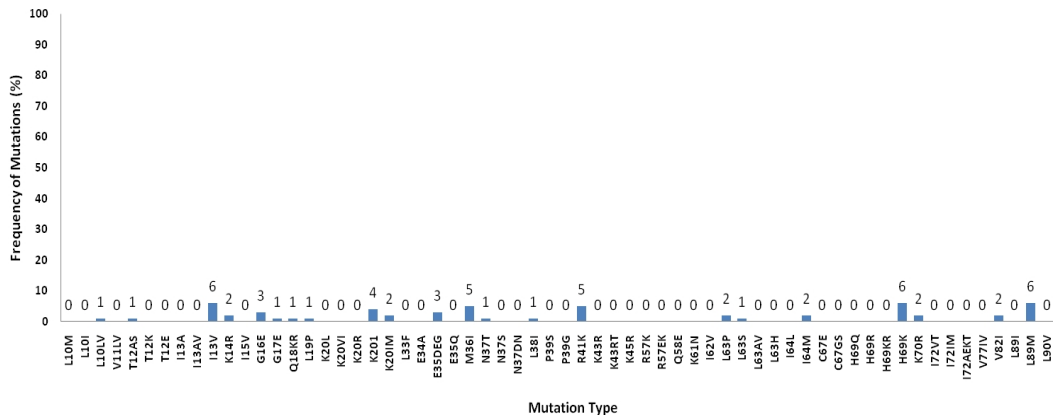
Fig. 4. Frequency of protease mutations in HIV-1 subtype CRF06_cpx isolates among antiretroviral treatment-naïve individuals
