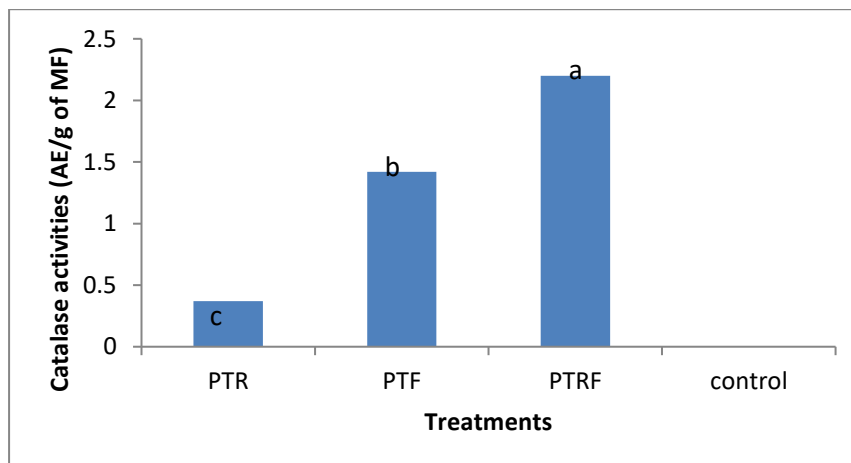
Fig. 3. Catalase activities in leaves of cotton plants treated or not with FOS from FOV
