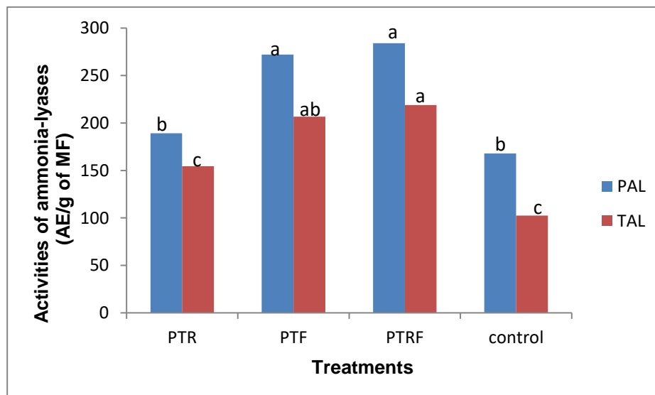
Fig. 1. Evolution of ammonia-lyase activity in leaves of cotton plants treated or not with FOS from FOV
