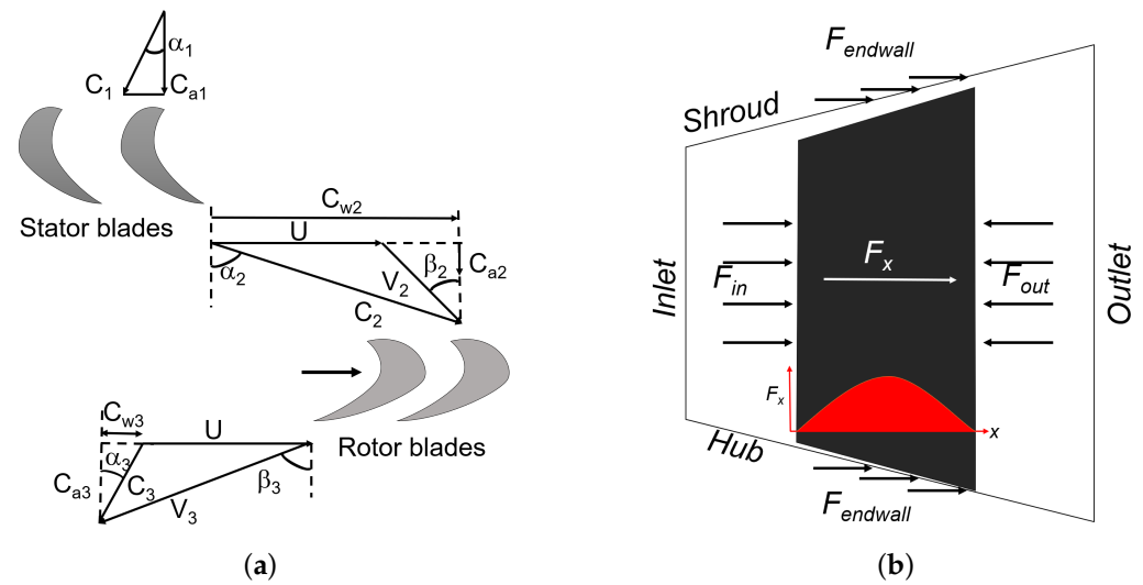
Figure 2. View of sample turbine blades. (a) Velocity triangle used in the mean line method. (b) Blade forces on the turbine blade.
