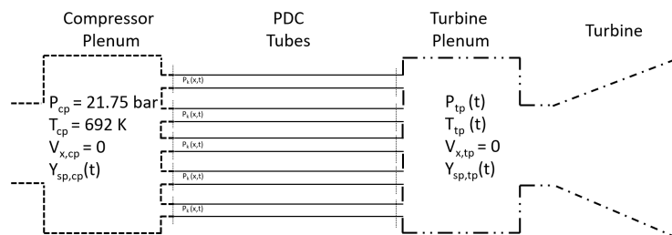
Figure 5. PDC setup.
