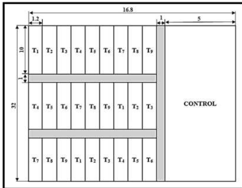
Fig. 2. Experimental layout
