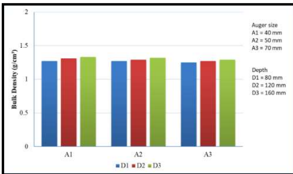
Fig. 6. Effect of auger size and depth on bulk density
