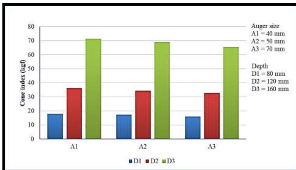
Fig. 7. Effect of auger size and depth on cone index
