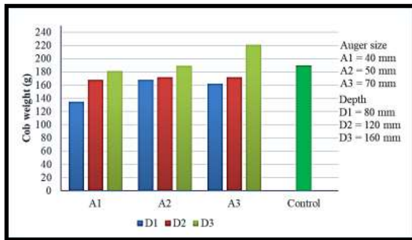
Fig. 11. Effect on cob weight for maize
