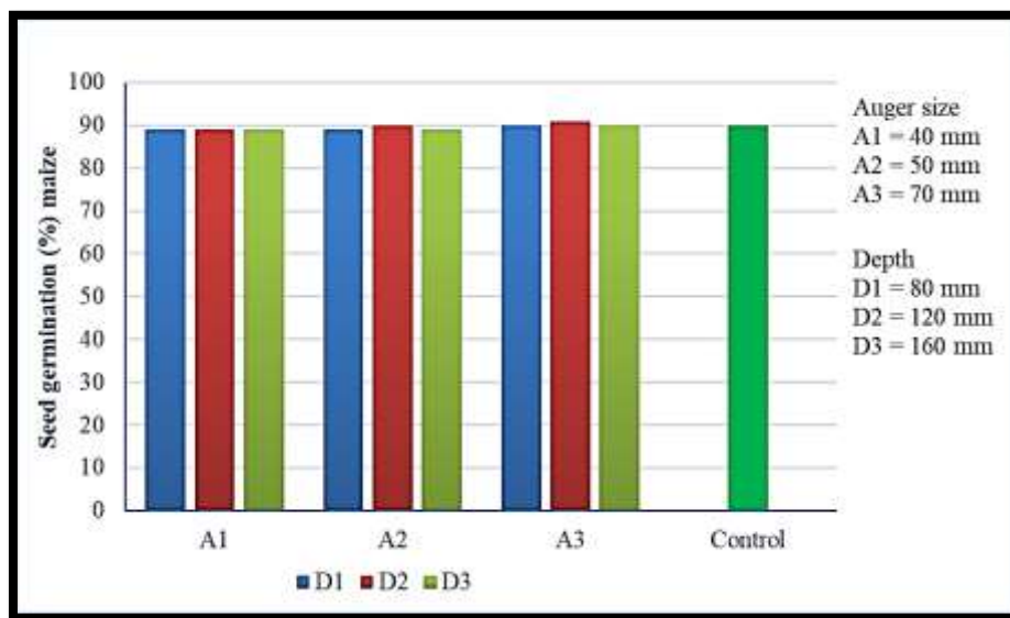
Fig. 8. Effect on germination for maize
