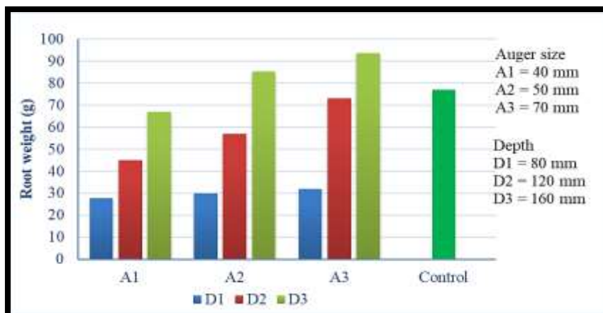
Fig. 10. Effect on root weight for maize
