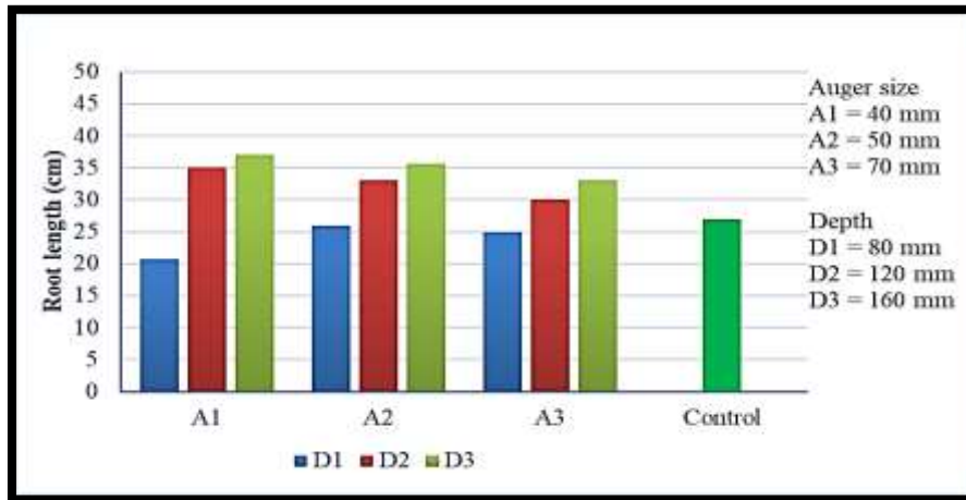
Fig. 9. Effect on root length for maize
