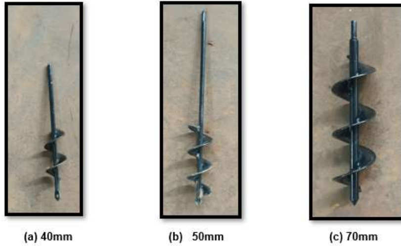
Fig. 1. Auger with different size
