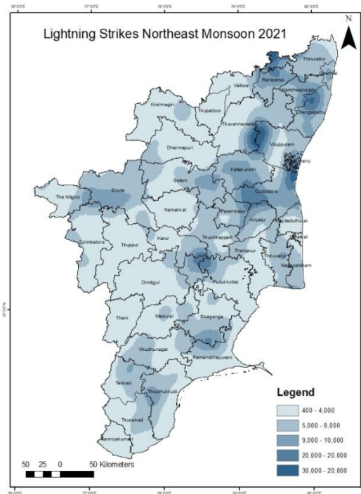
Fig. 3. Lightning strikes over Tamil Nadu during NEM 2021
