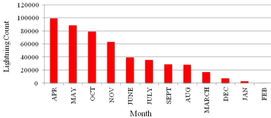
Fig. 10. Cloud to Ground lightning activity over Tamil Nadu during 2019 – 2021
