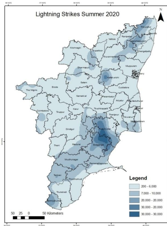
Fig. 8. Lightning strikes over Tamil Nadu during Summer (Pre monsoon) 2020
