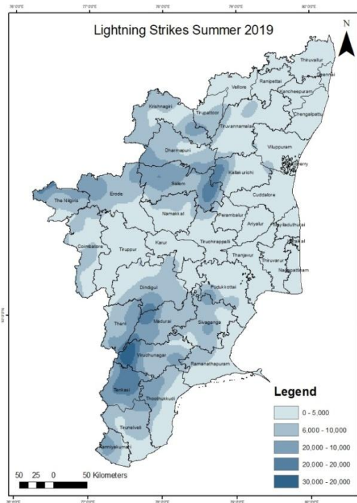
Fig. 7. Lightning strikes over Tamil Nadu during Summer (Pre monsoon) 2019
