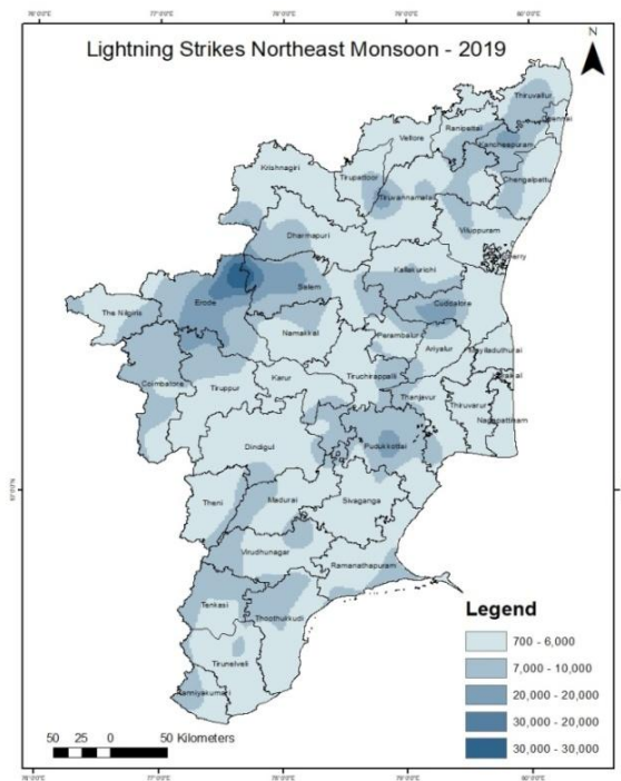
Fig. 1. Lightning strikes over Tamil Nadu during NEM 2019
