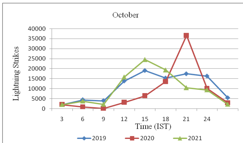
Fig. 11. Diurnal pattern of Cloud to Ground flash occurrences during October
