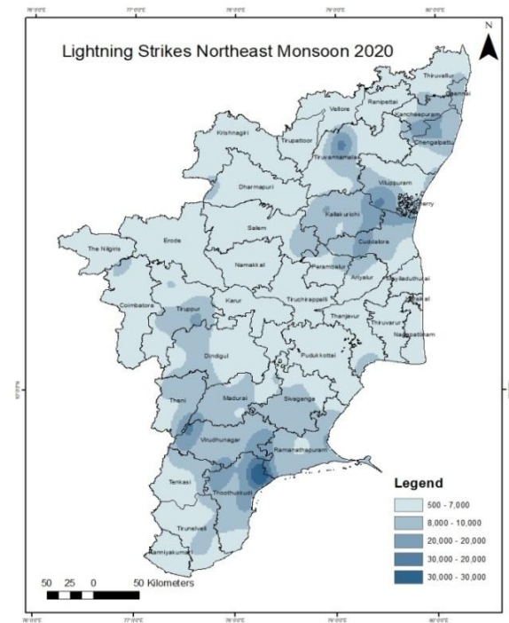
Fig. 2. Lightning strikes over Tamil Nadu during NEM 2020
