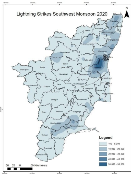
Fig. 5. Lightning strikes over Tamil Nadu during SWM 2020
