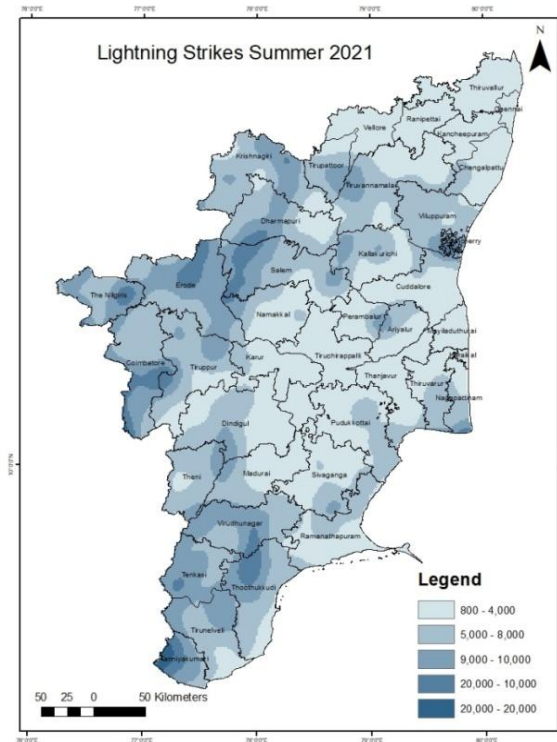
Fig. 9. Lightning strikes over Tamil Nadu during Summer (Pre monsoon) 2021
